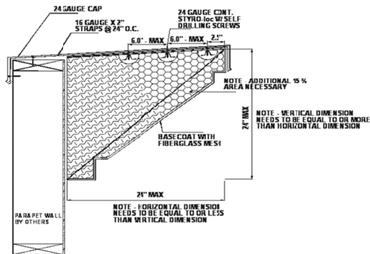
FIGURE 3—SPACING OF STYRO-LOC INSERTS
