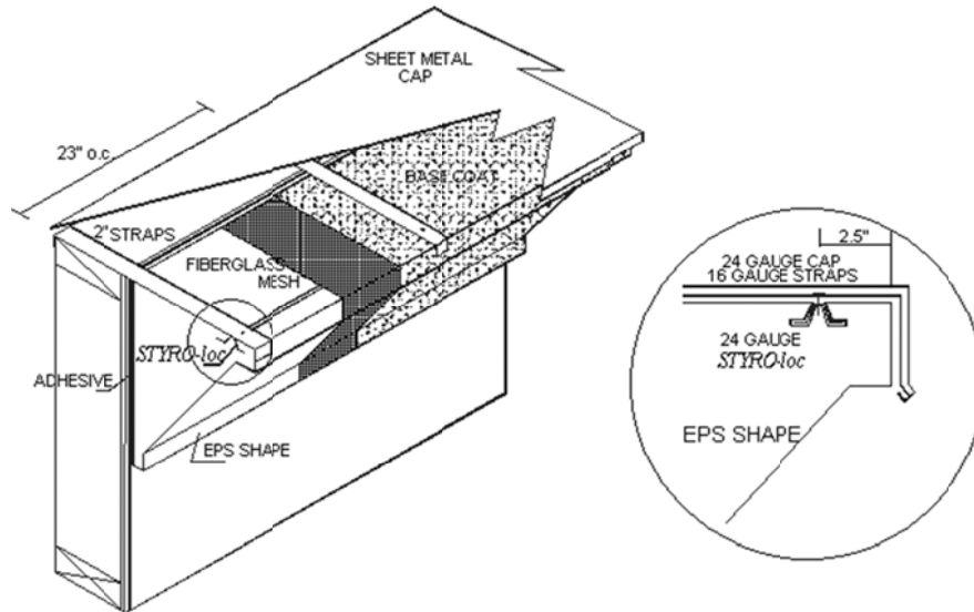
FIGURE 1—STYRO-LOC SYSTEM
