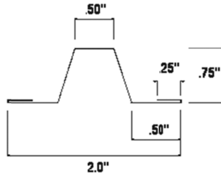
FIGURE—2 STYRO-LOC INSERT
